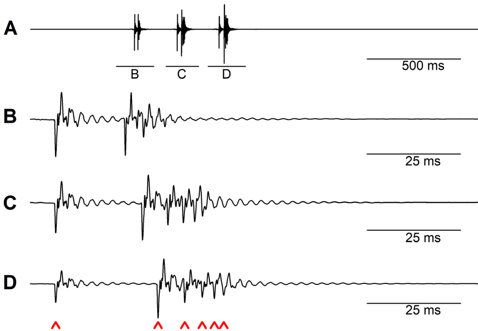
Fig. 1. Oscillograms at different time resolutions showing the amplitude modulation pattern of a Besdolus ventralis male call. A, an entire call; B, the first beat group of the call shown in A; C, the second beat group of the call shown in A; D, the third beat group of the call shown in A, red /\ symbols point toward individual beats. (Amplitude is normalised to 100% in each oscillogram.)
