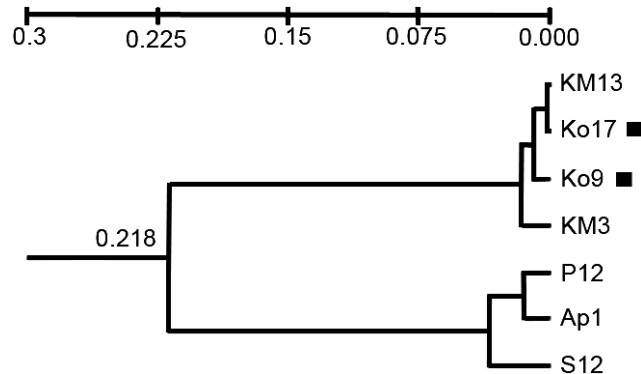
Fig. 2. UPGMA clustering of Nei's original genetic distances between populations of Daphnia atkinsoni and D. bolivari . The morphological D. bolivari populations are marked with black squares (Ko17 and Ko9).
